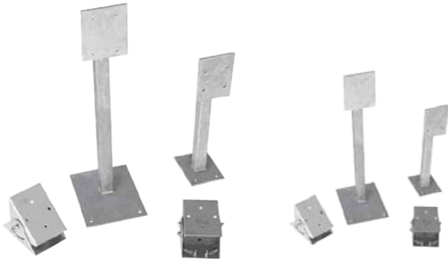
M1-Mounting bracket (long) w/ half-pan/tilt
